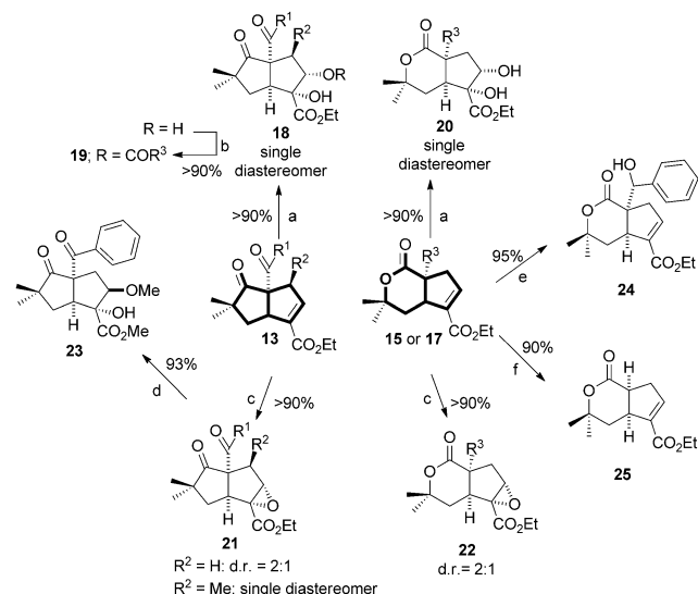
Scheme 2. Functionalization of the bicyclic scaffolds. Reaction conditions: a) OsO 4 , NMO, THF/H 2 O, RT; b) R 3 COCl or R 3 CO 2 H, RT; c) mCPBA, RT; d) pTSA, MeOH, 45 °C, 3 days; e) DibalH, -78 °C; f) pTSA, (CH 2 OH) 2 , RT. NMO = N-methylmorpholine N-oxide, mCPBA = meta -chloroperoxybenzoic acid, pTSA = para -toluenesulfonic acid, DibalH = diisobutylaluminum hydride.
